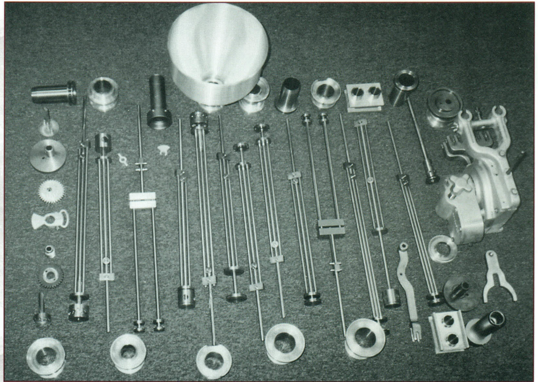
Stainless Steel plungers for every configuration are standard components. Plungers are interchangeable with most makes of depositors in the industry.
